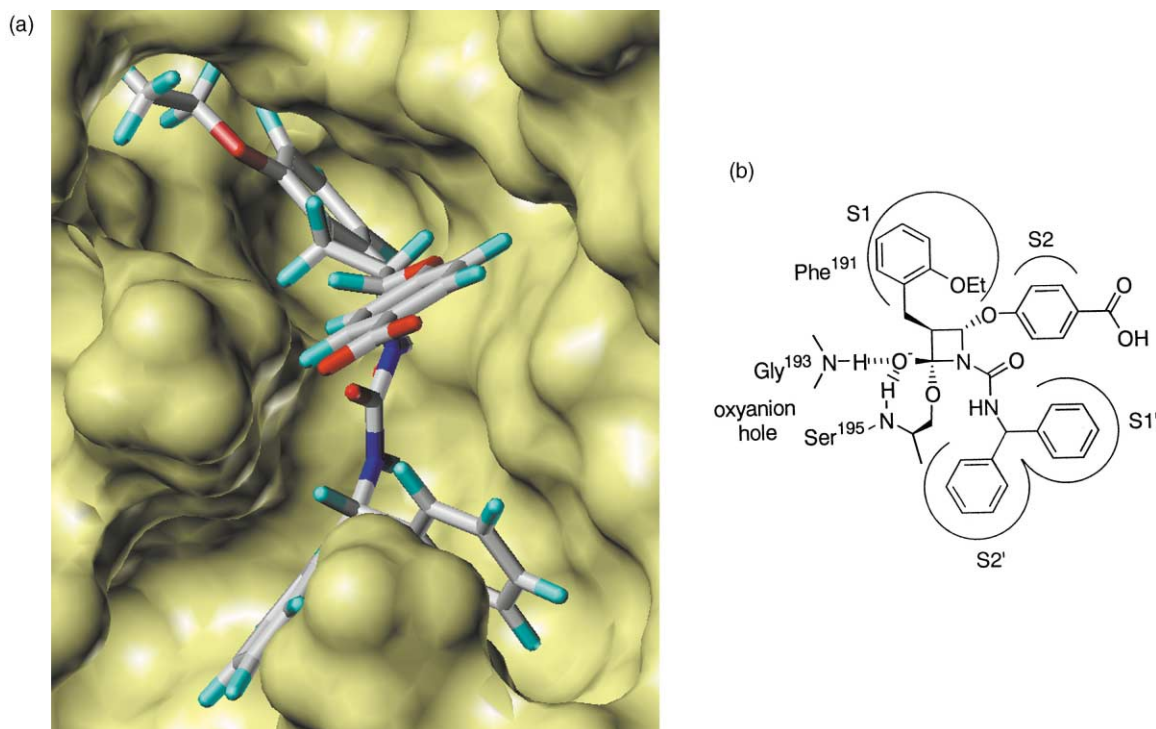
Figure 4. Docking model of inhibitor 23 into human chymase: (a) surface representation; (b) schematic drawing.
