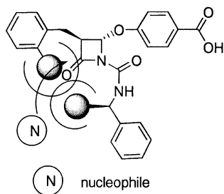
Figure 2. Schematic drawing of steric effects at 1- and 3-positions.
