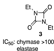
Figure 1. Design of 3-benzylazetidine-2-one-based human chymase inhibitor.
