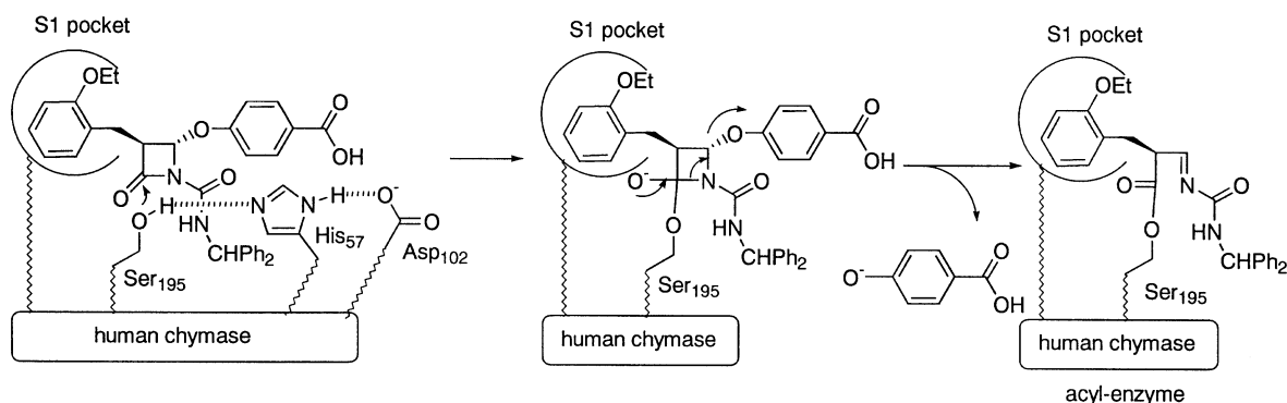
Figure 3. Proposed mechanism for inhibition of human chymase by compound 23 .
